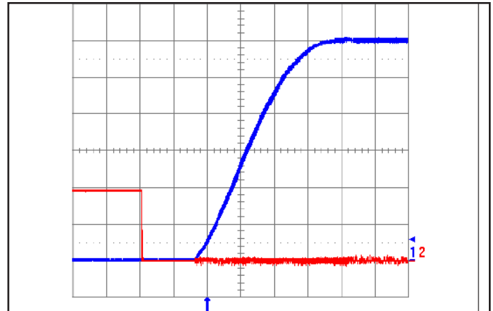
Figure 10: Turn-on transient at zero load and 3 mF output capacitance (2 ms/div). Input voltage pre-applied. Ch 1: Vout (2 V/div), Ch 2: ON/OFF input (2 V/div).
