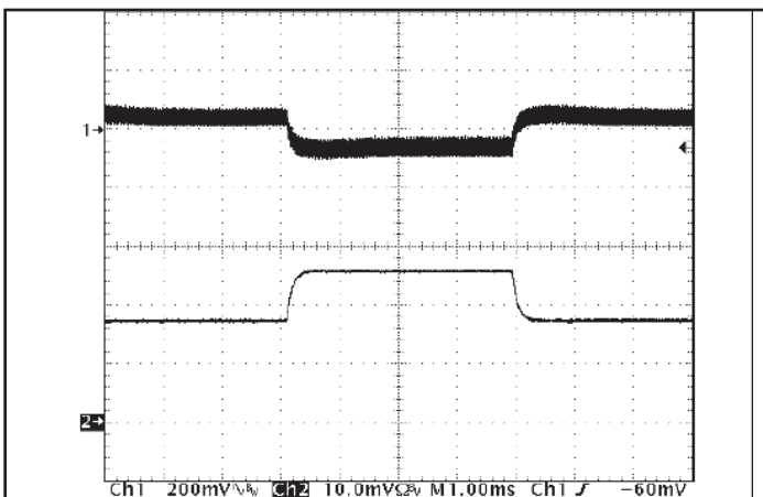
Figure 11: Output voltage response to step-change in load current (50%-75%-50% of Iout(max); dI/dt = 0.1 A/μs). Load cap: 15 μF tantalum cap and 1 μF ceramic cap. Top trace: Vout (200 mV/div), Bottom trace: Iout (5 A/div).
