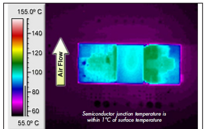
Figure 6: Thermal plot of converter at 16 A load current (192 W) with 55 °C air flowing at the rate of 200 LFM. Air is flowing across the converter from pin 3 to pin 1 (nominal input voltage).
