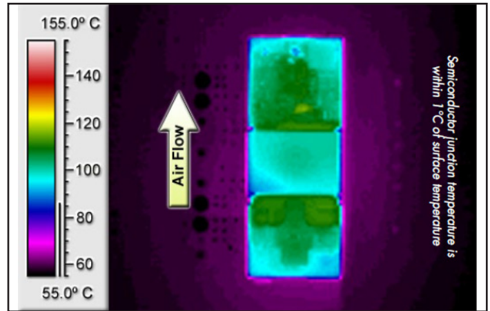
Figure 8: Thermal plot of converter at 16 A load current (192 W) with 55 °C air flowing at the rate of 200 LFM. Air is flowing across the converter from output to input (nominal input voltage).
