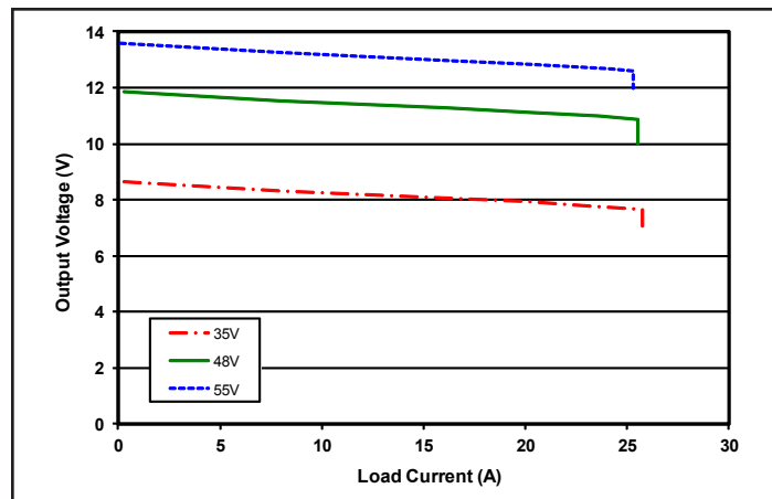
Figure 16: Output voltage vs. load current for different input voltages showing typical current limit curves.
