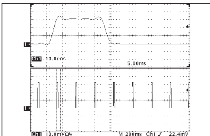
Figure 17: Load current ( 10\ \text{A/div} ) as a function of time when the converter attempts to turn on into a 1\ \text{m}\Omega short circuit. Top trace ( 5.0\ \text{ms/div} ) is an expansion of the on-time portion of the bottom trace.
