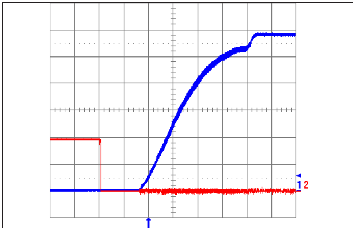
Figure 9: Turn-on transient at 50% load (resistive load) and 3 mF output capacitance (2.0 ms/div). Input voltage pre-applied. Ch 1: Vout (2 V/div), Ch 2: ON/OFF input (2 V/div).
