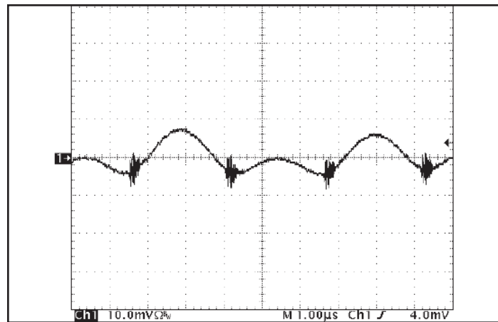
Figure 14: Input reflected ripple current, i_s , through a 10\ \mu\text{H} source inductor, using a 47\ \mu\text{F} electrolytic input capacitor ( 5\ \text{mA/div} ). See Figure 12.
